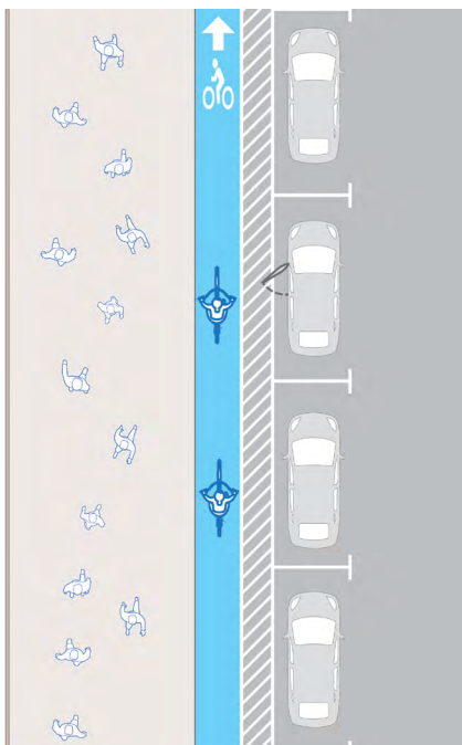
Figure 26. Buffer between cycle lane and parking lane using on-street markings using paint.
