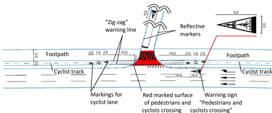
Example of marking of footpaths and cyclist tracks on crossing of the road
