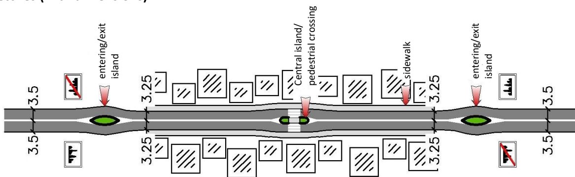
Example of road elements within the built-up areas
