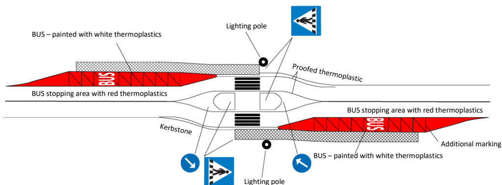
Good example of pedestrian crossing and BUS stops
