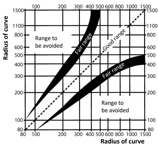
The combination of radii for rural roads
